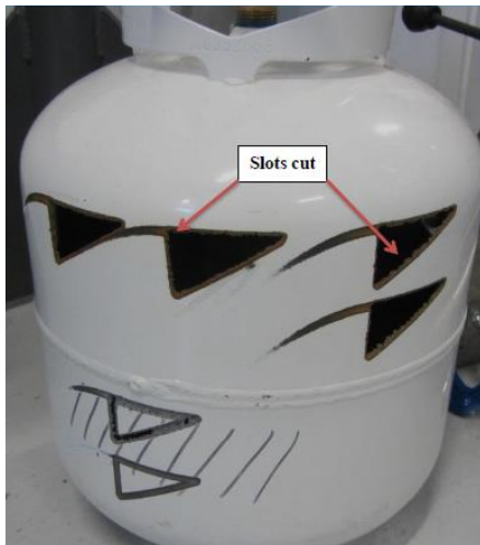
Figure 10 – Photograph of sections of cylinder selectively cut out using FPWJ.
