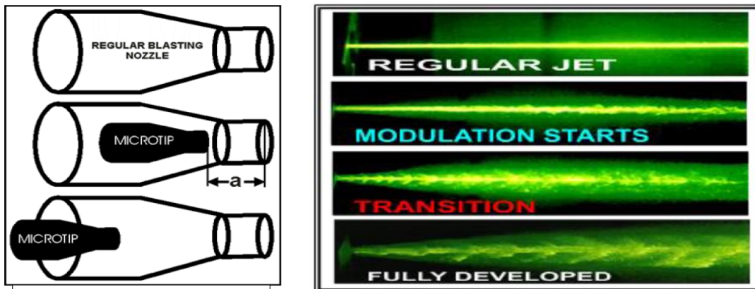
Figure 1 Positioning of Ultrasonic transducer. Figure 2 – High speed photographs of a traditional water jet and the establishment of a FPWJ.
