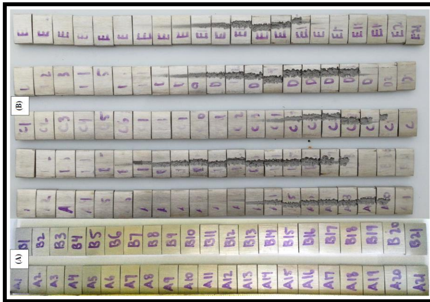
Figure 7 – Photograph of samples following drop test procedure for mass loss determinations. (A) before, (B) after.
