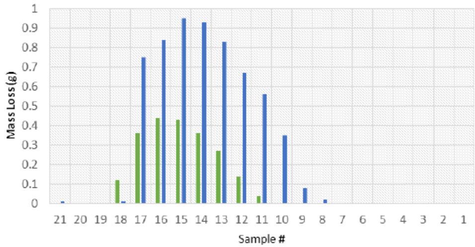
Figure 9 – Mass loss for angled and perpendicular jets.
