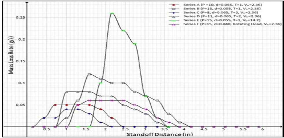
Figure 8 – Drop-test generated graph. Mass loss rate vs standoff distance for various operating conditions
