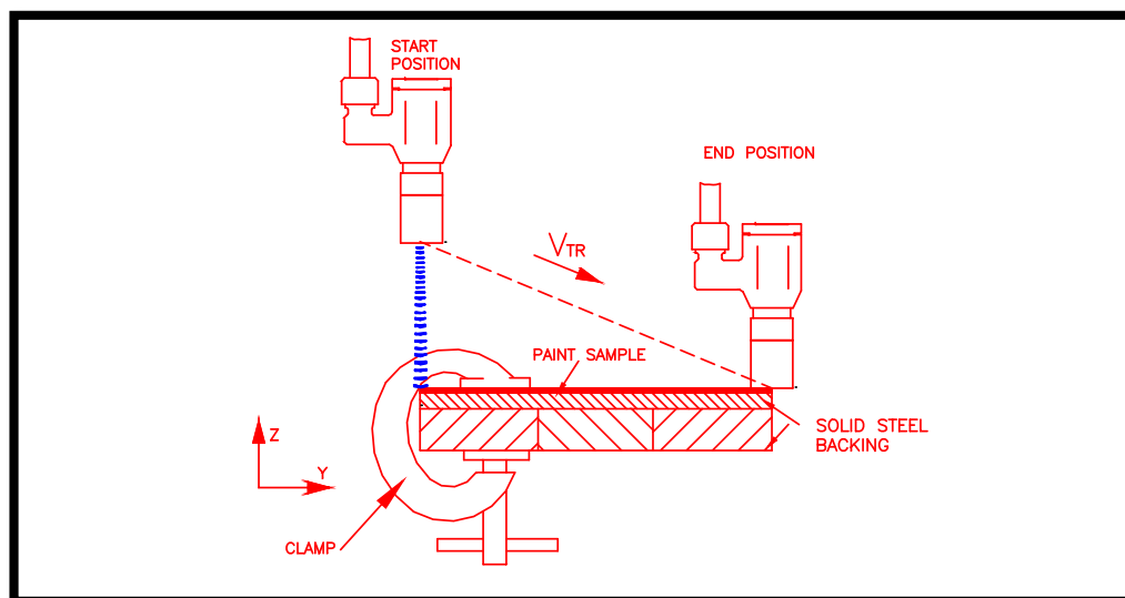
Figure 3 – Illustration of ‘drop test’.
