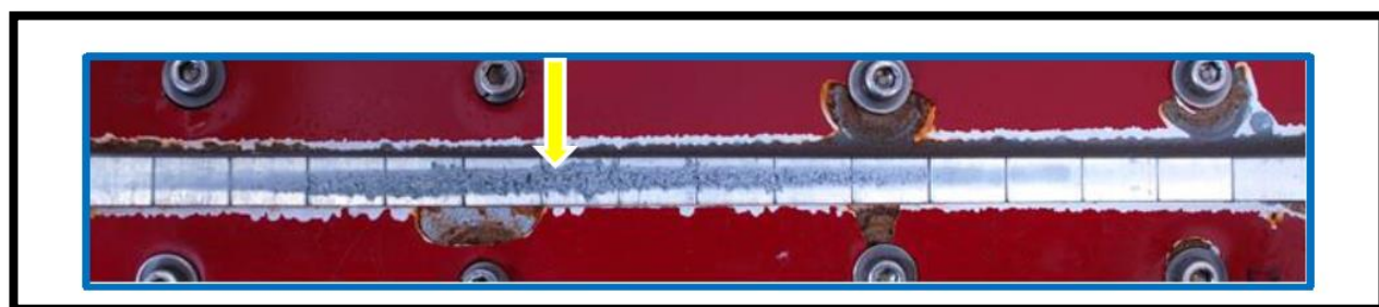
Figure 4 – Example of the stripe pattern from a ‘drop test’. Yellow arrow indicates optimum standoff.
