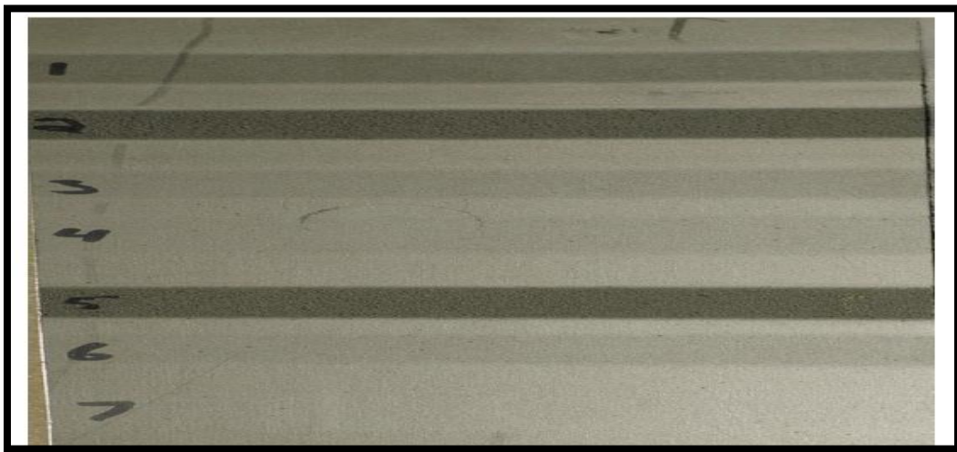
Figure 6 – Shows the banding effect from changing parameters, against a series of trial runs. Darker bands show greater degrees of erosion that correspond to more overlap (equivalent to jet dwell time).
